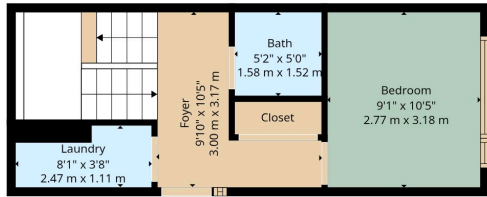
1st Floor
