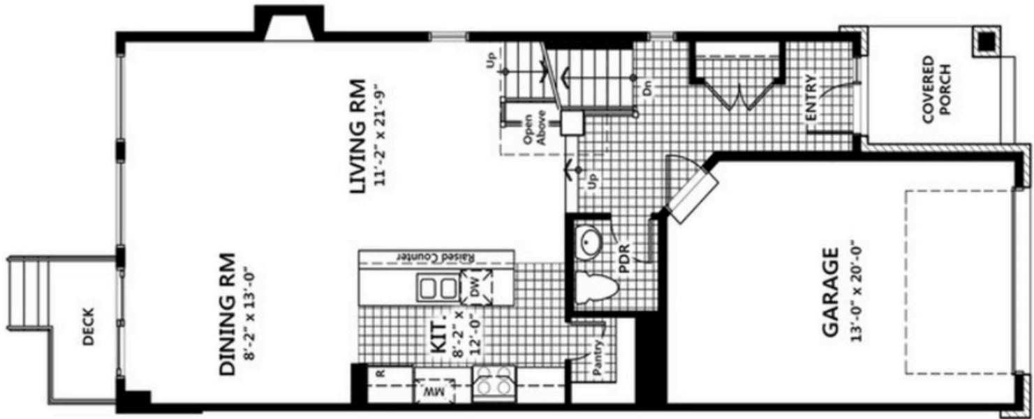
FIRST FLOOR
