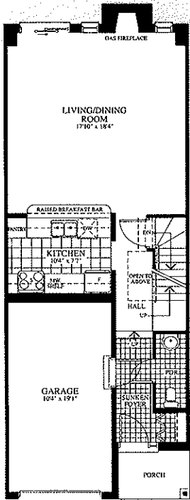
Ground floor
